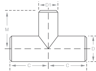
Reducer Tee
