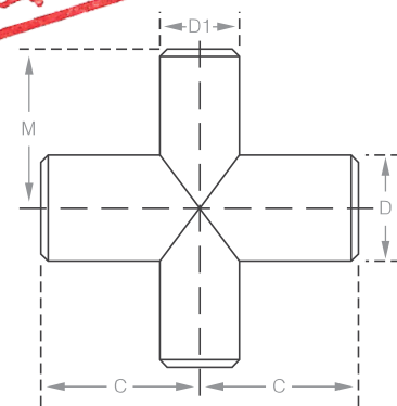
Reducer Cross
