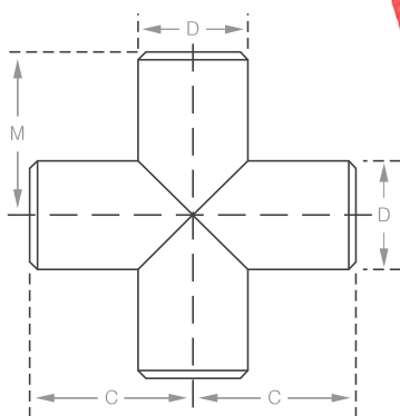
Cross Tee
